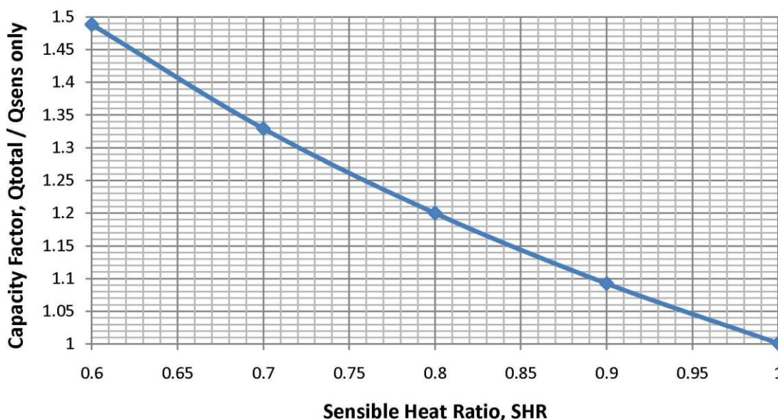
FIGURE 2 Total Cooling Capacity Factor vs SHR
